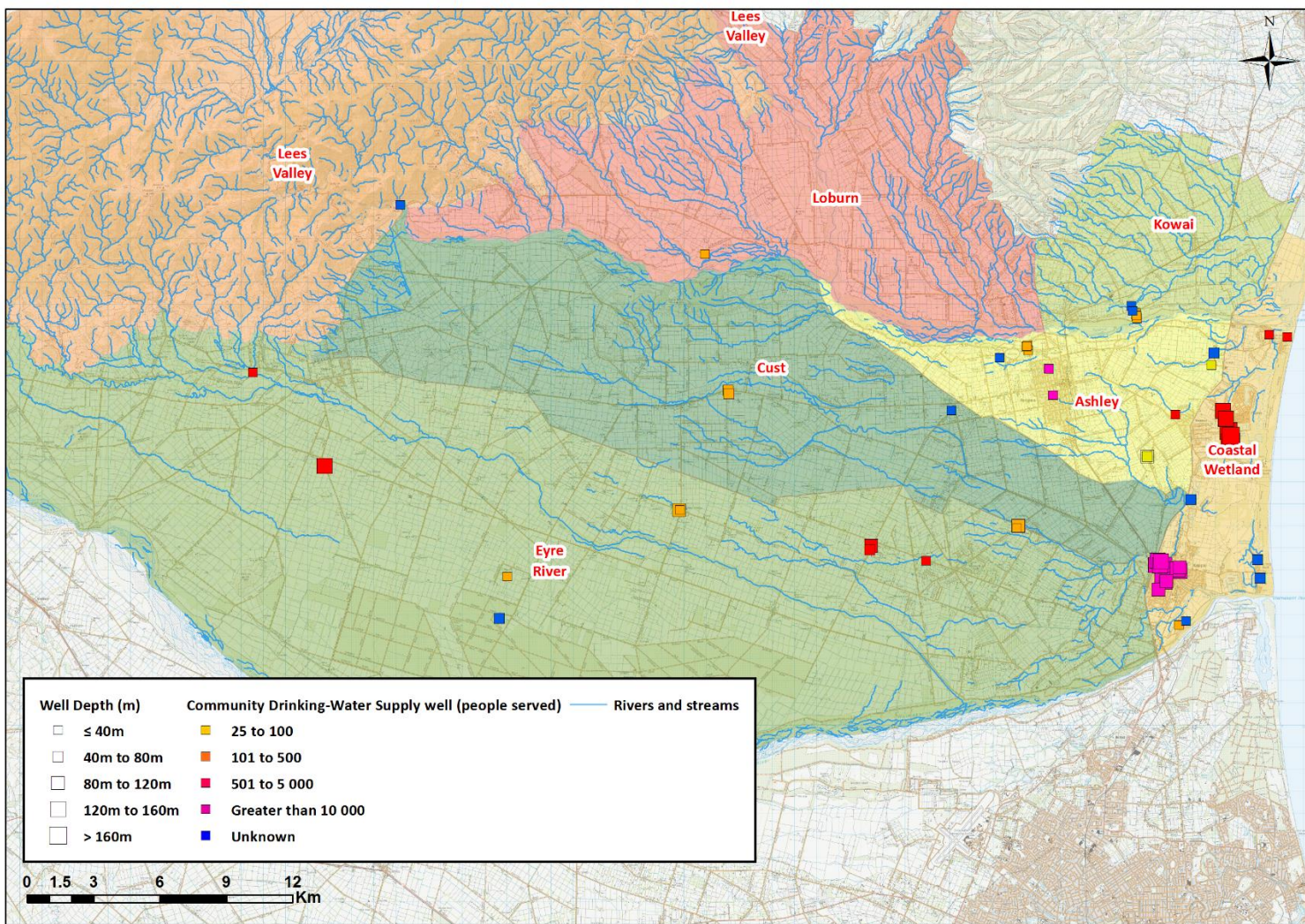
Figure 5-5 Distribution of community drinking water supply wells
