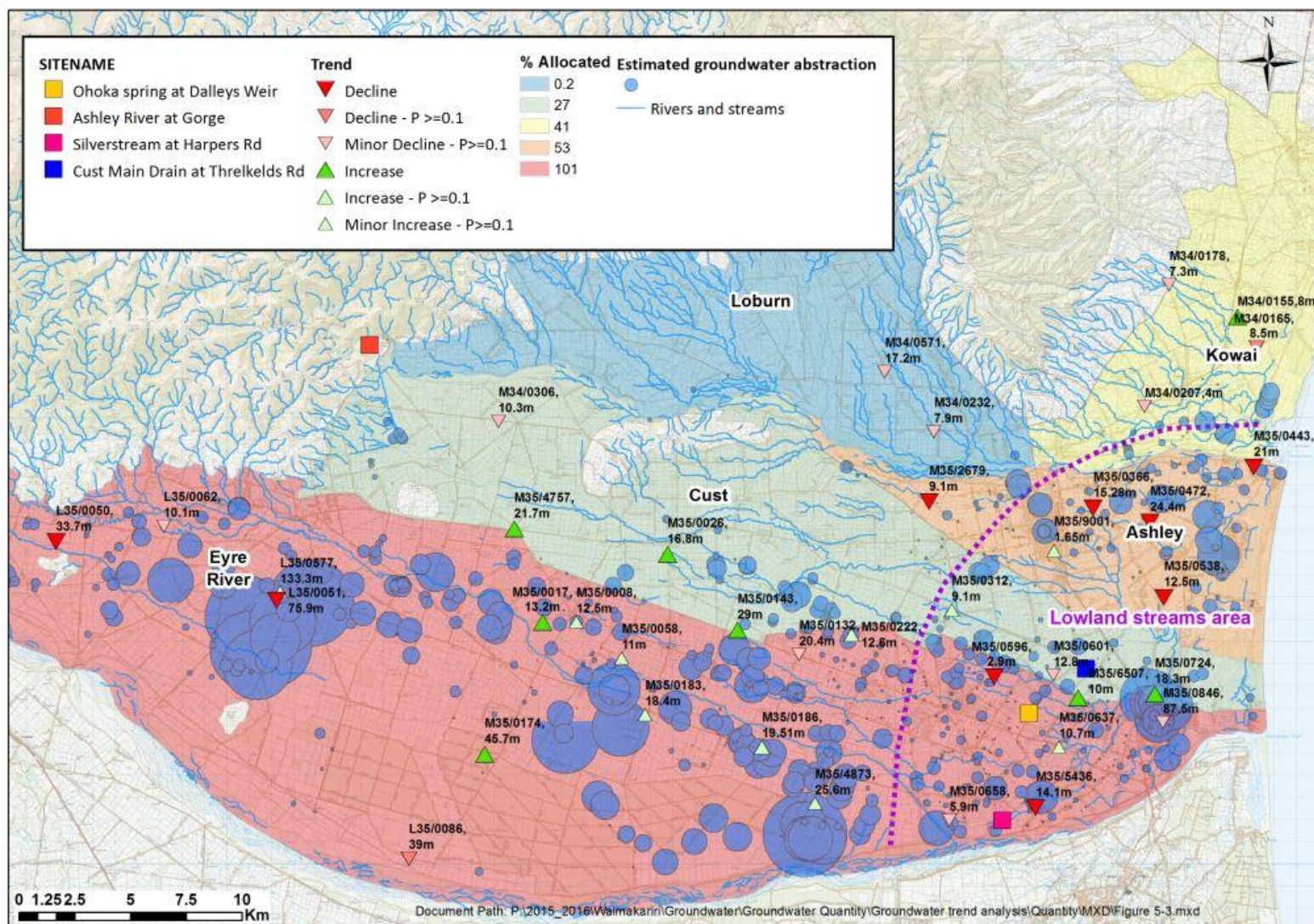
Figure 5-3 Long-term groundwater level trend (post WIL Scheme) based on Seasonal Mann-Kendall analysis
