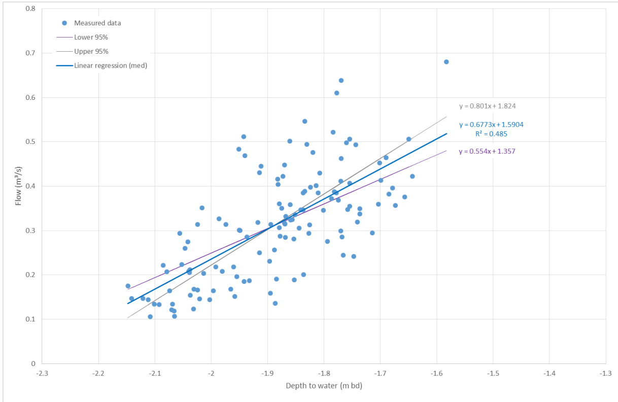
Figure 10-3 M35/5463 groundwater level vs Silverstream flow
