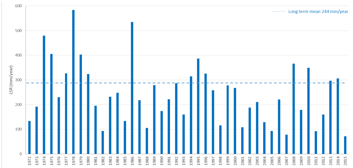
Figure 3-2 Annual Land Surface Recharge over time 12
