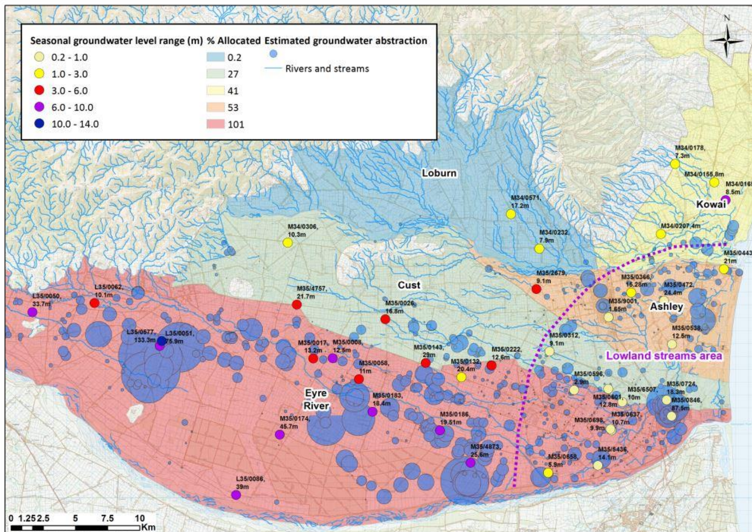
Figure 5-1: Seasonal groundwater level range (well depths labelled)
