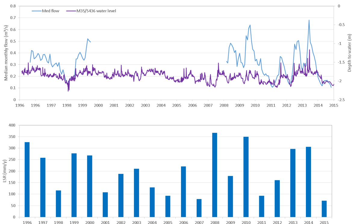
Figure 5-6 M35/5436 water level, median monthly Silverstream flow and annual LSR
