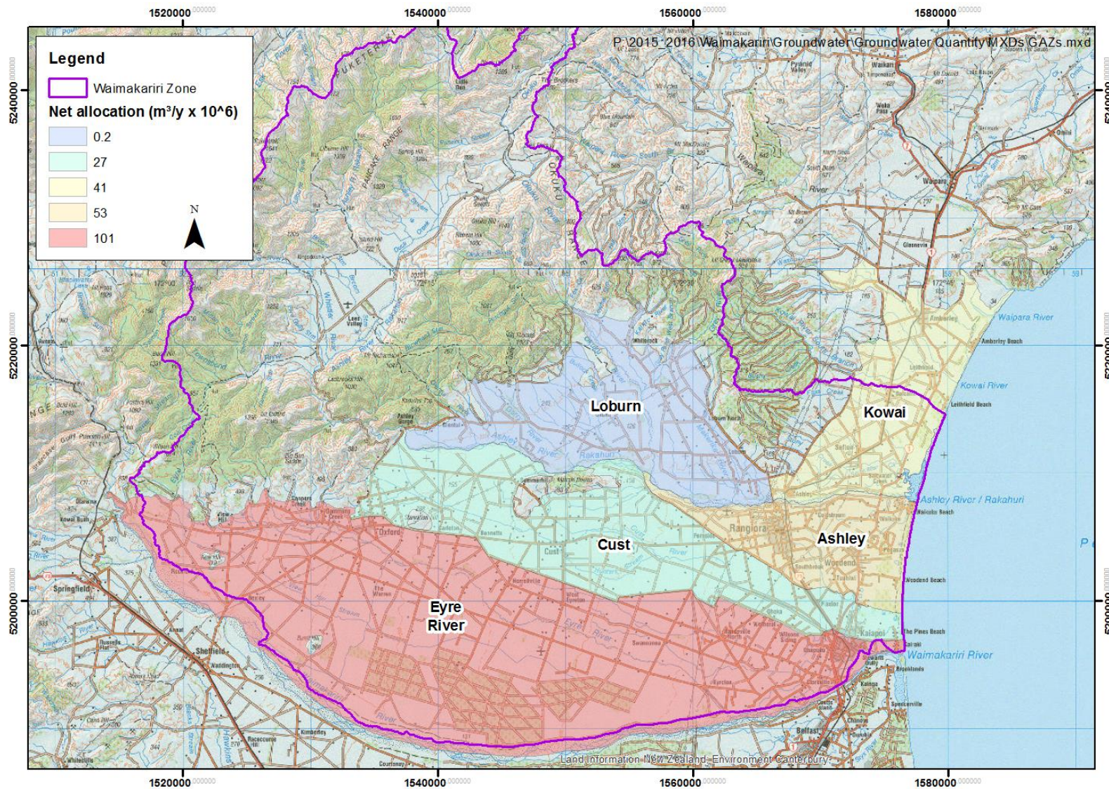
Figure 2-1 Groundwater allocation zones
