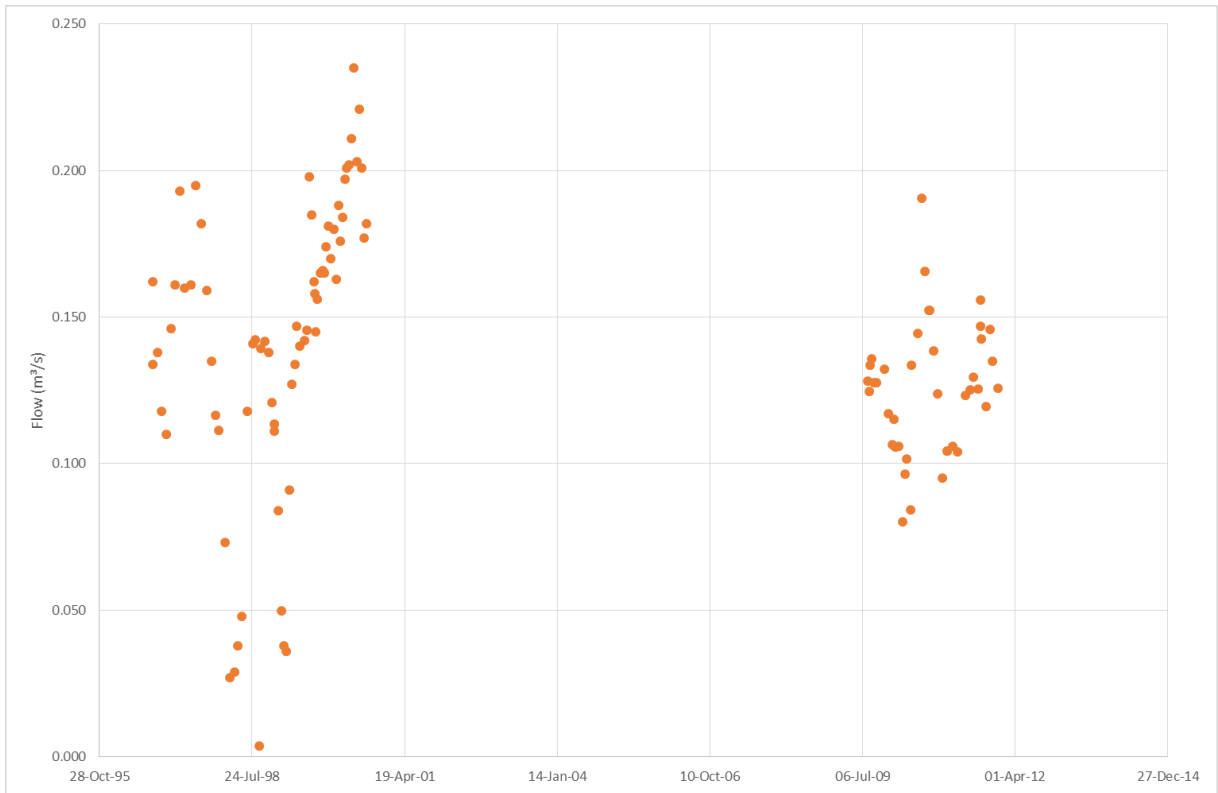
Figure 10-2 Taranaki Creek flow gauging data
