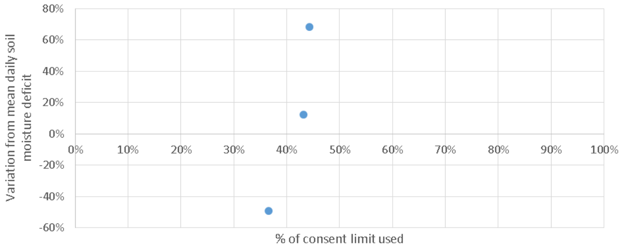
Figure 2-3 Water use versus deviation from mean soil moisture deficit
