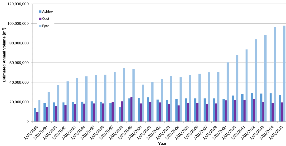
Figure 2-4 Groundwater allocation over time
