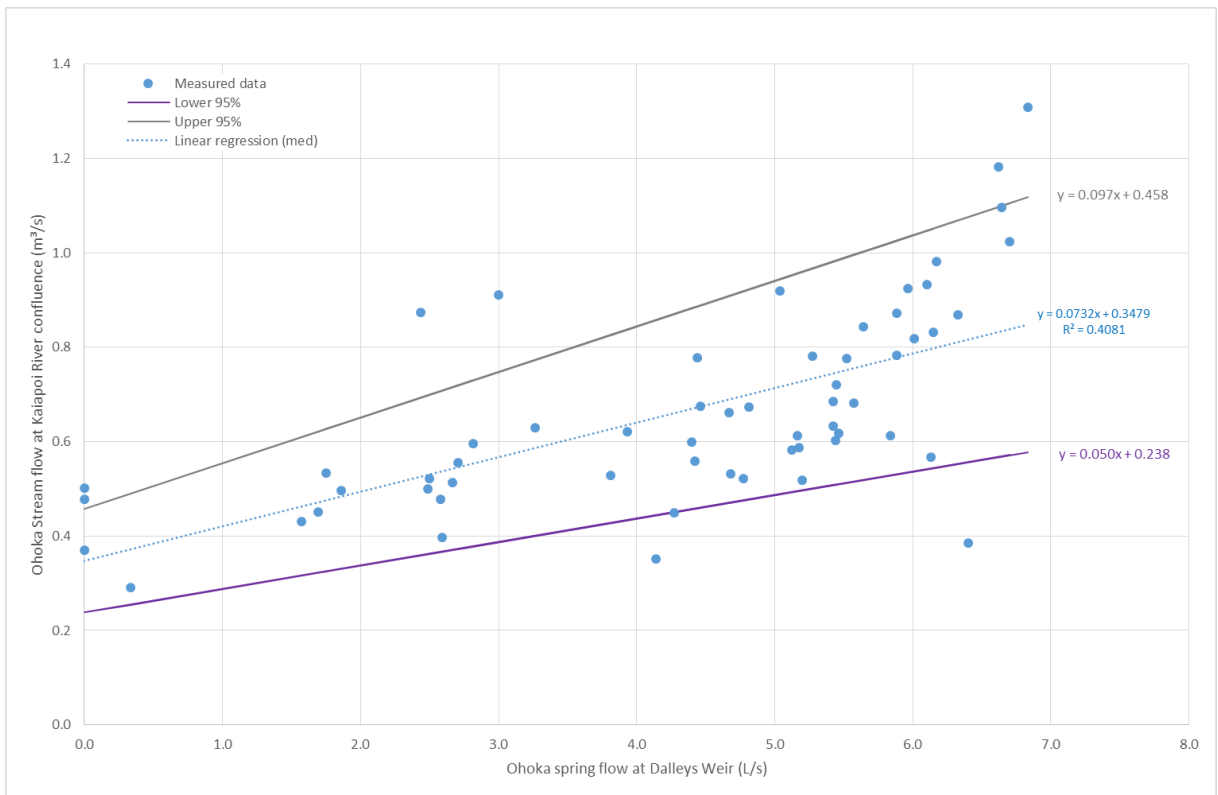
Figure 10-4 Ohoka Stream flow vs Dalley's Weir spring flow
