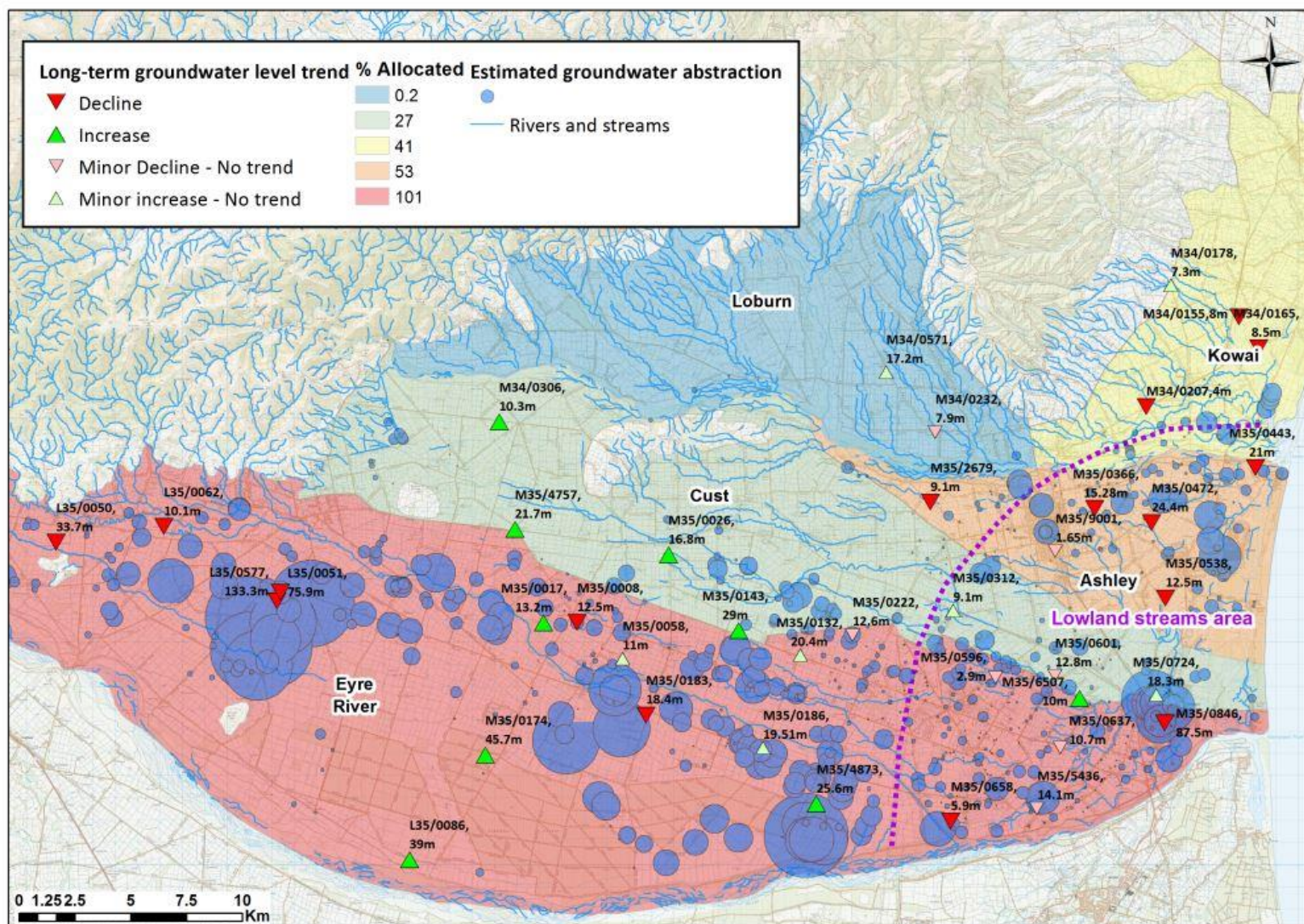
Figure 5-2: Long-term groundwater level trend based on linear regression analysis (well depths labelled)
