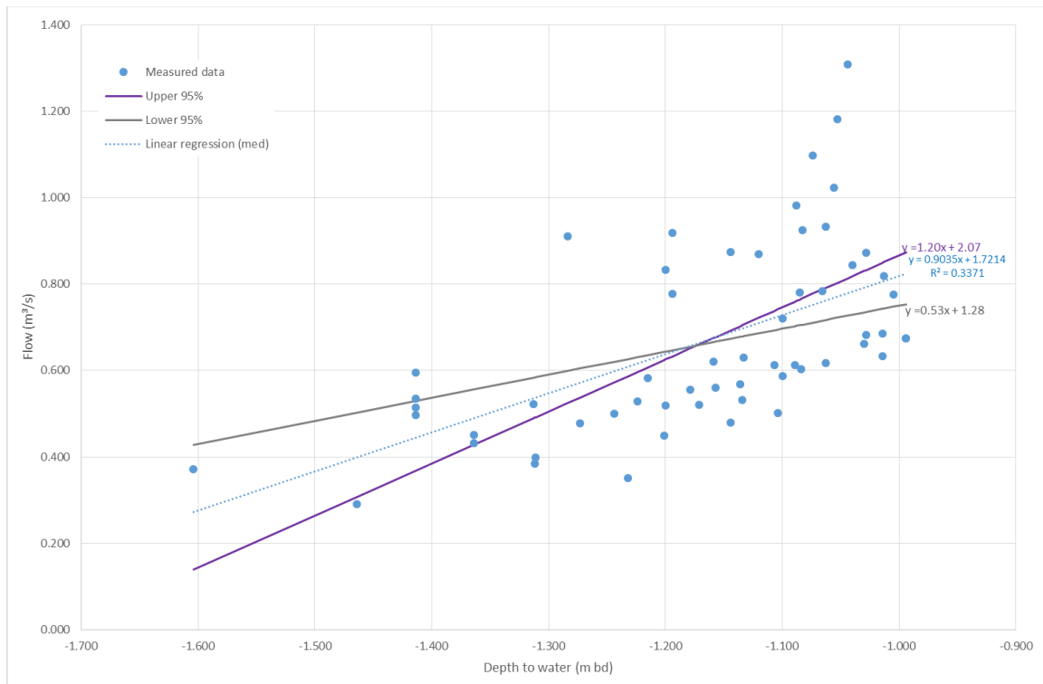
Figure 10-5 M35/0596 groundwater level vs Ohoka Stream flow
