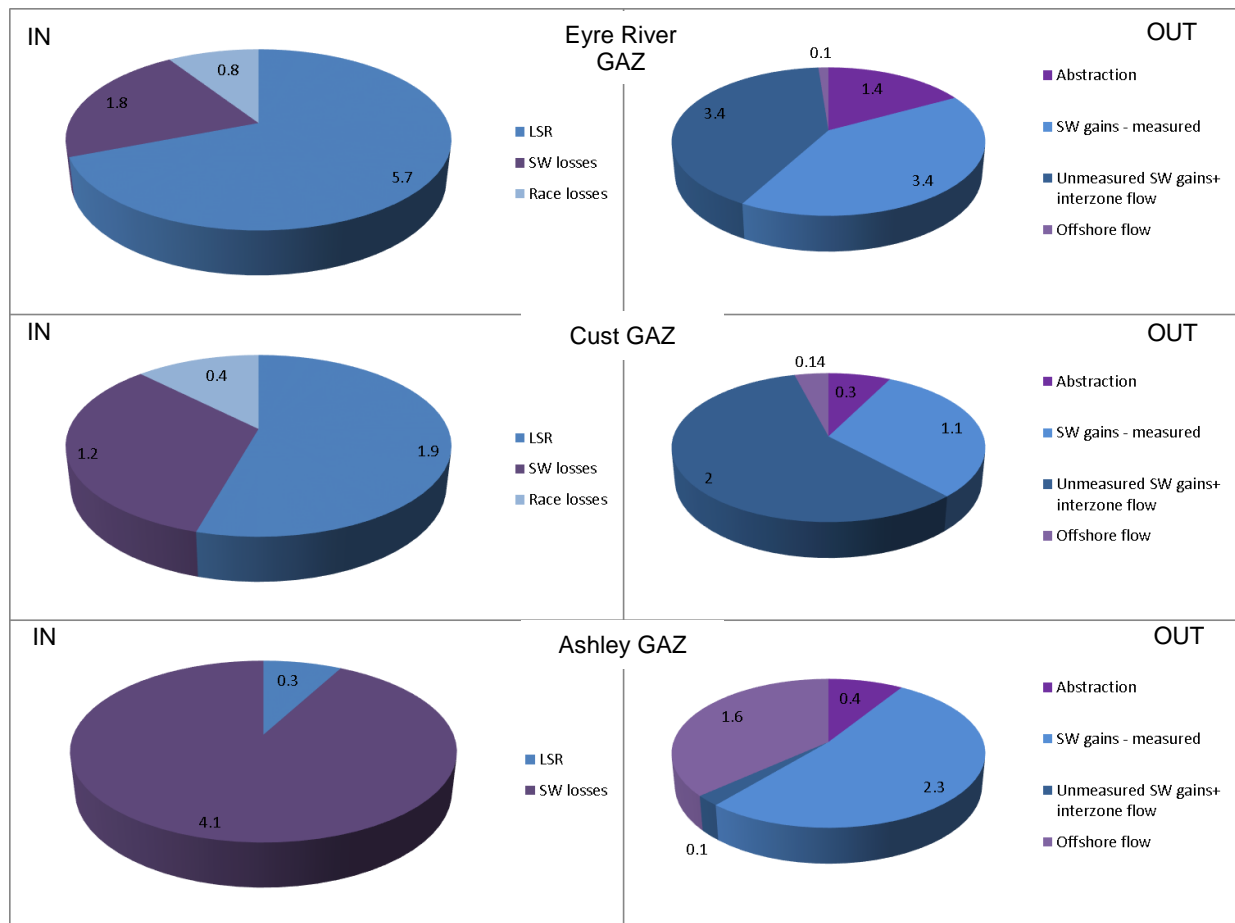
Figure 3-1 Long term average groundwater budgets for Eyre, Cust and Ashley GAZs (m 3 /s)
