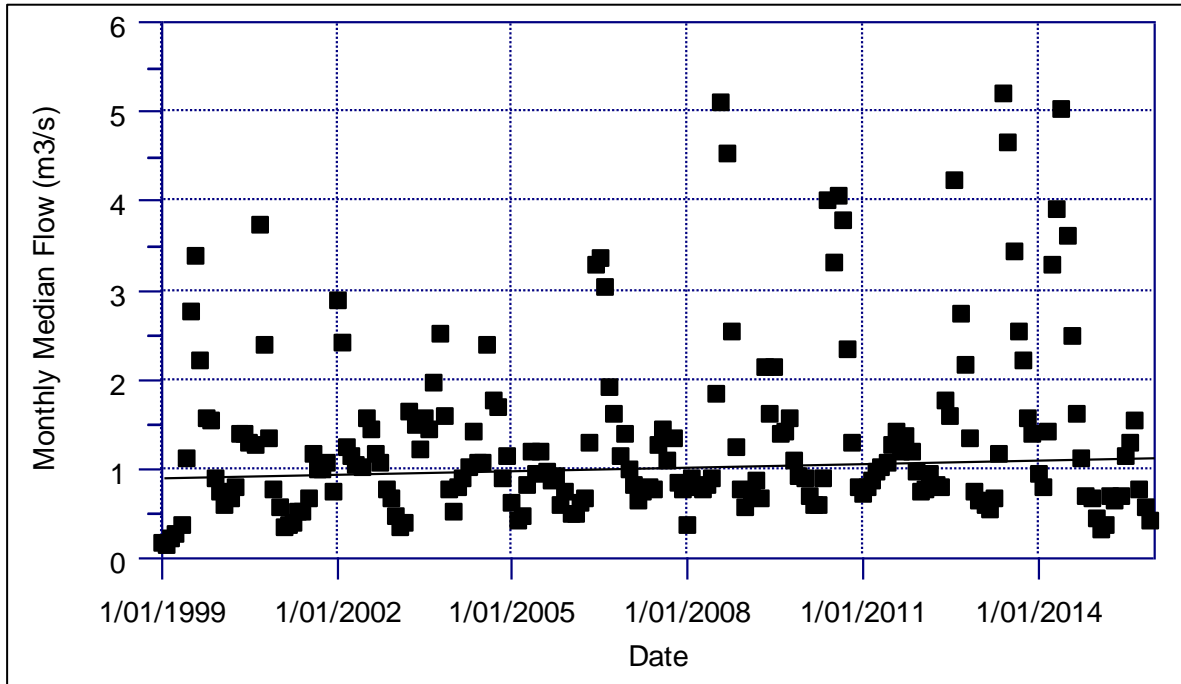
Figure 10-6: Seasonal Mann-Kendal trend analysis for Cust Main Drain (from 1999 to 2015)
